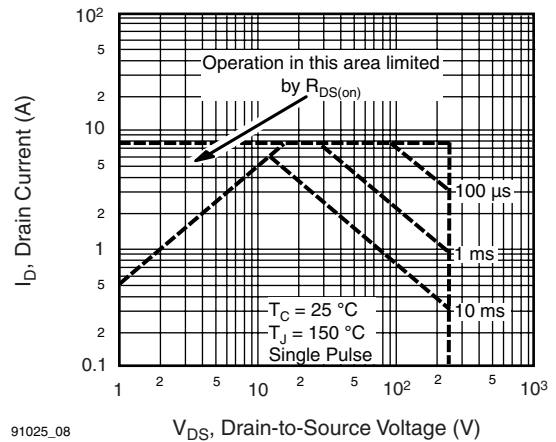
Fig. 3 - Fig. 8 - Maximum Safe Operating Area
